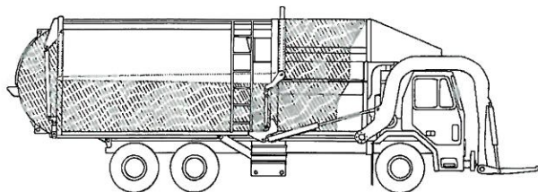
LOWER COMPARTMENT
